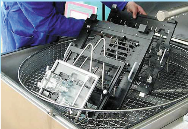
Cleaning with STAR 100 – plastic parts
